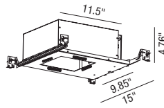
Shallow Housing
