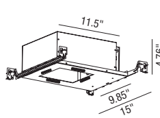
Shallow Housing
