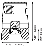
Narrow Housing
