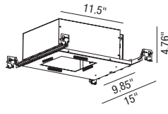
Shallow Housing
