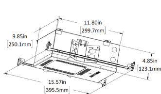
Shallow Housing
