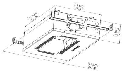
Shallow Housing
