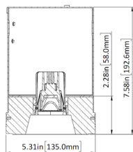
Narrow Housing
