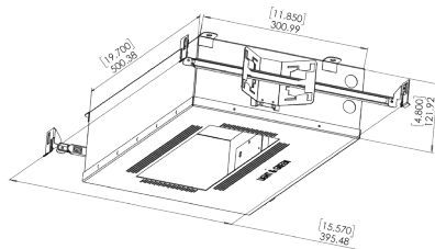
Shallow Housing
