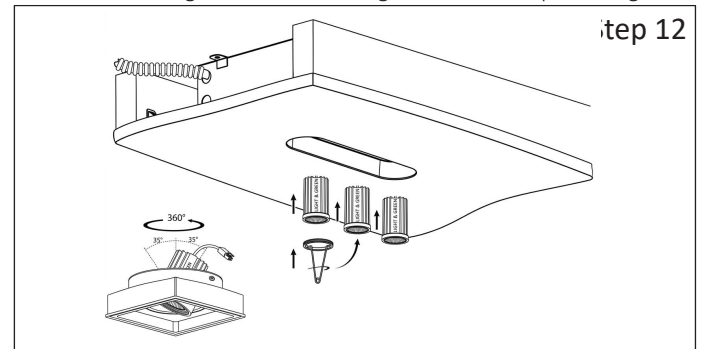
Step 12 - Replace Fixture Ring and Install LED Light:
