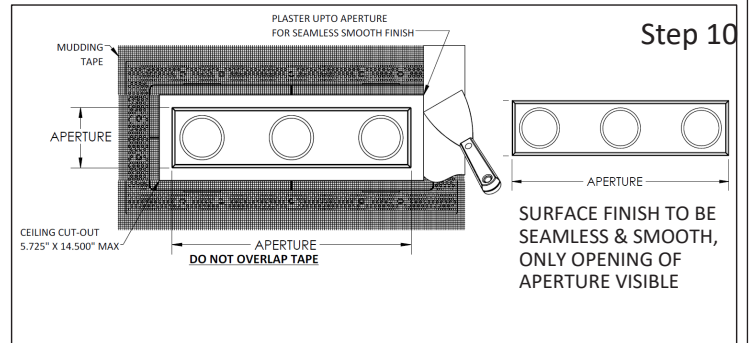
Step 10 - Plastering Ceiling Cut-Out with fixture and Paint
